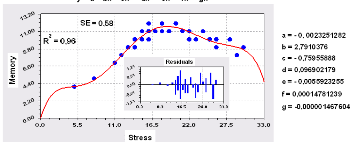
Figure 2. Graphic representation relation between stress (x) on the memory (y) in study population y = a + bx + cx^2 + dx^3 + ex^4 + fx^5 + gx^6
